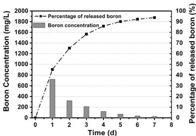
Fig. 2 Concentration of boron released each day from the scaffolds into a simulated body fluid (SBF), and the cumulated concentration of boron released (as a fraction of the boron concentration in the as-prepared scaffold)
