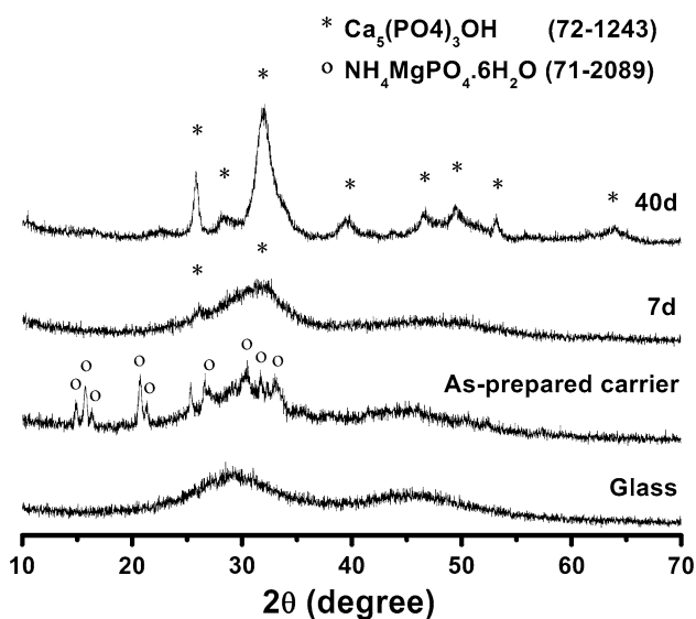
Fig. 5 XRD patterns of the starting borate glass powder, the as-prepared borate glass scaffold, and the borate glass scaffold after immersion for 7 and 40 days in a SBF
