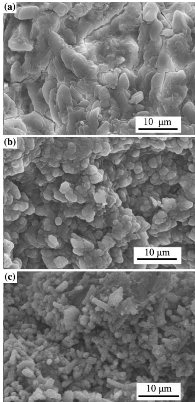
Fig. 6 Microstructure of the as-prepared scaffold (a), and the scaffold after immersion for 7 days (b) and 40 days (c) in a SBF
