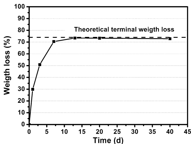
Fig. 3 Weight loss of bioactive borate glass scaffolds as a function of immersion time in a SBF. The ‘theoretical’ weight loss of the scaffolds is shown by the dashed line
